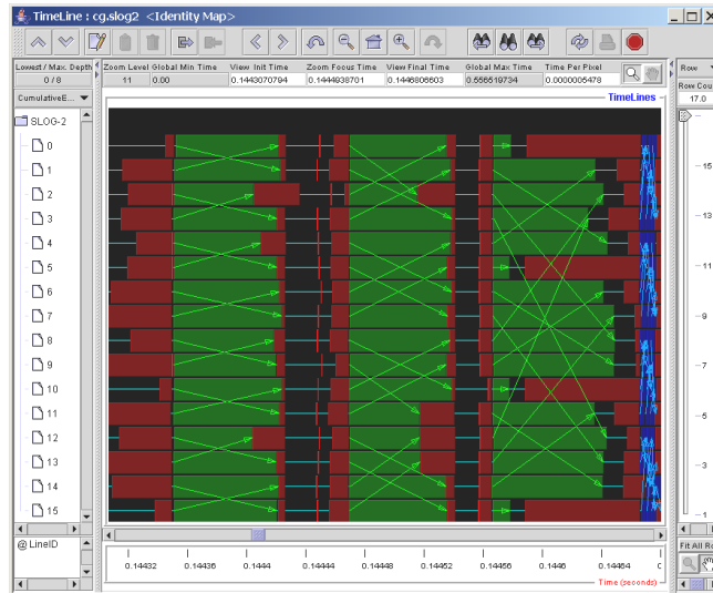
Fig. 6. Jumpshot timeline view of NPB CG benchmark
