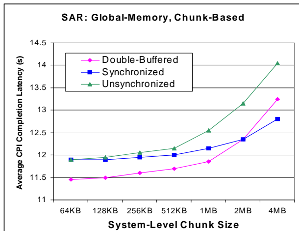
Figure 1- Variants of Parallel SAR Algorithm
